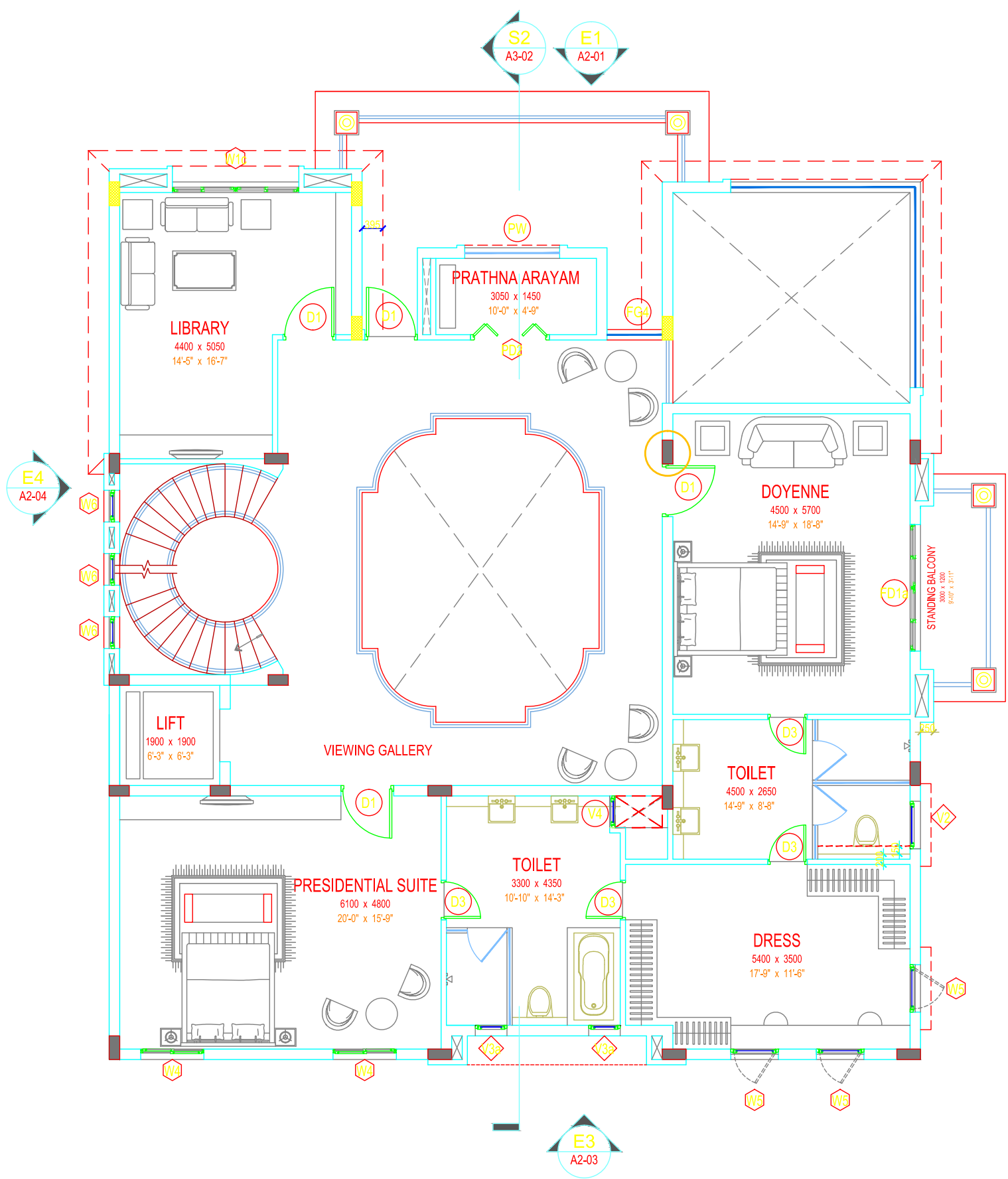
VILLA : 55/56 First Floor Plan
