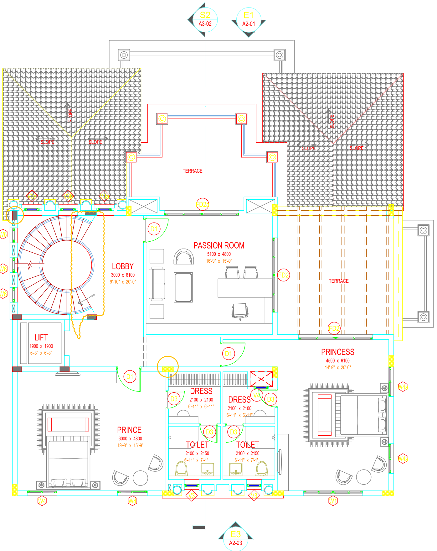
VILLA : 55/56 Second Floor Plan
