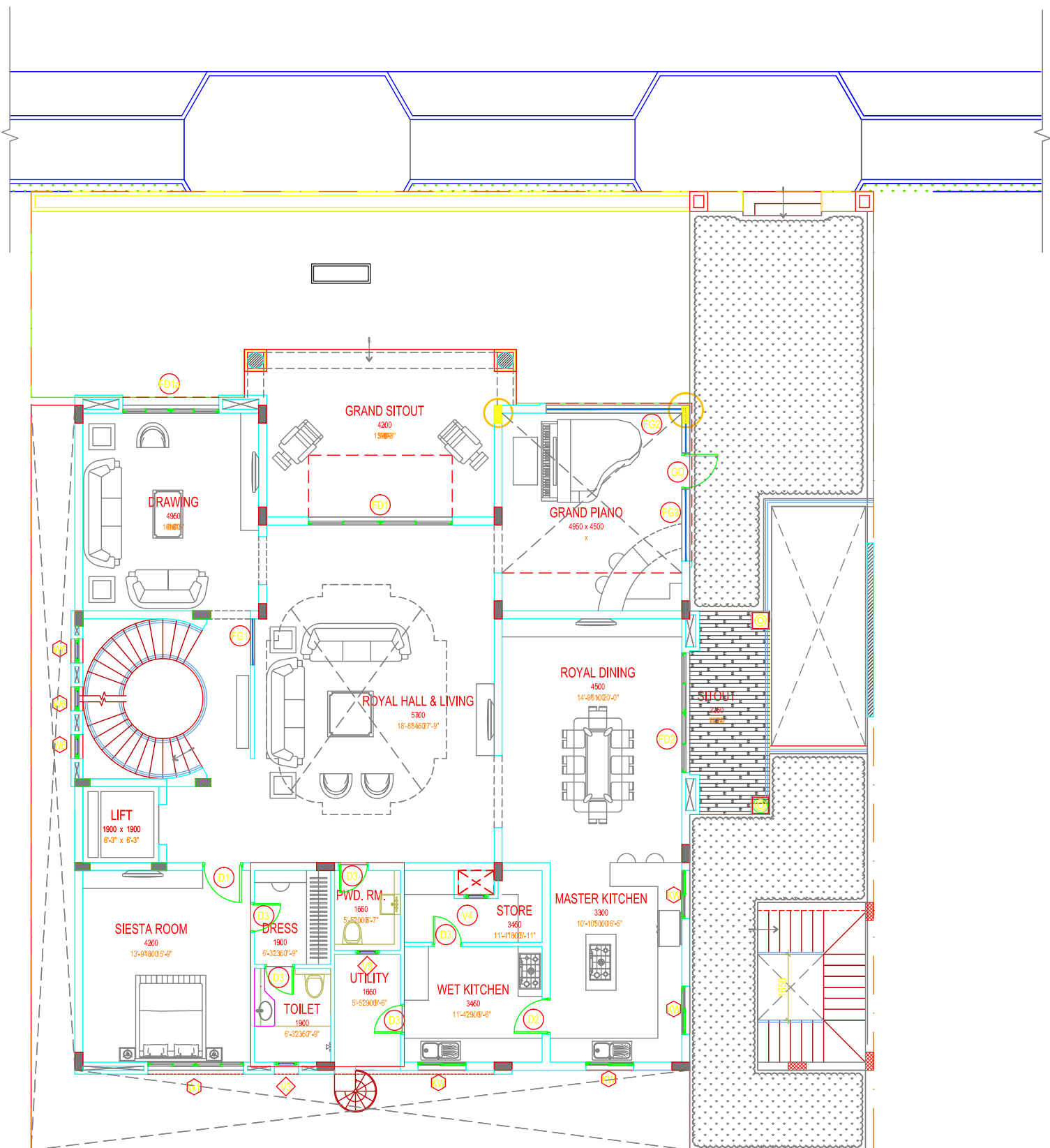
VILLA : 55/56 Ground Floor Plan
